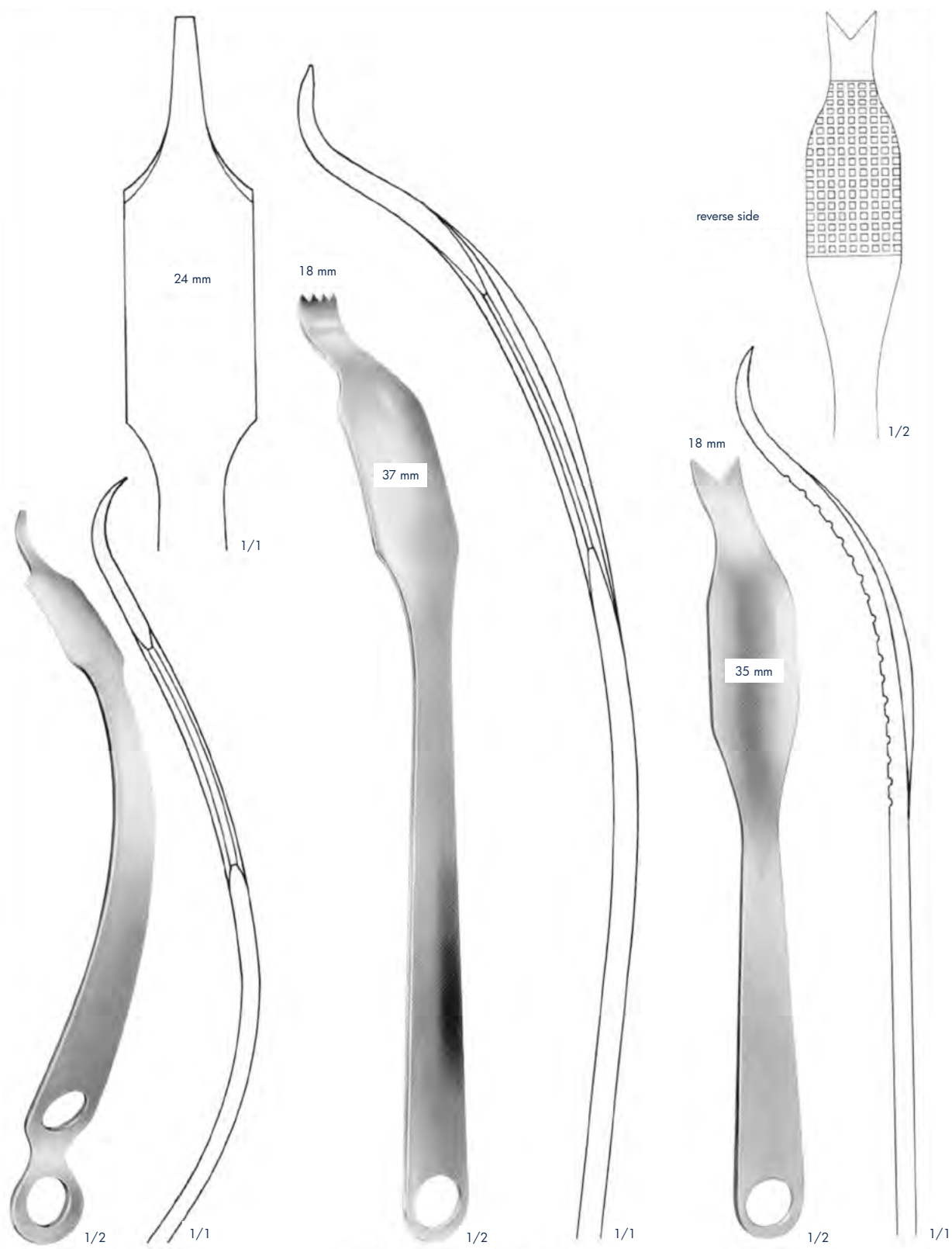
HOHMANN-ALDINGER ASI150480 270 mm
