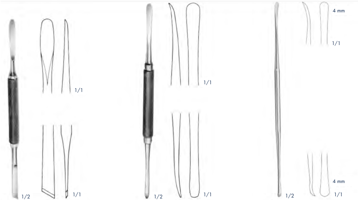
MEAD ASI190681 sharp 165 mm
