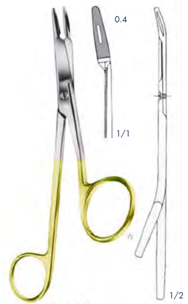
GILLIES ASI170339 160 mm
