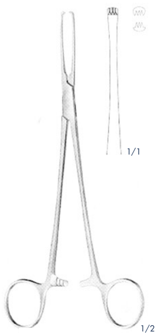
JUDD-ALLIS ASI230318 3 x 4 teeth 195 mm
