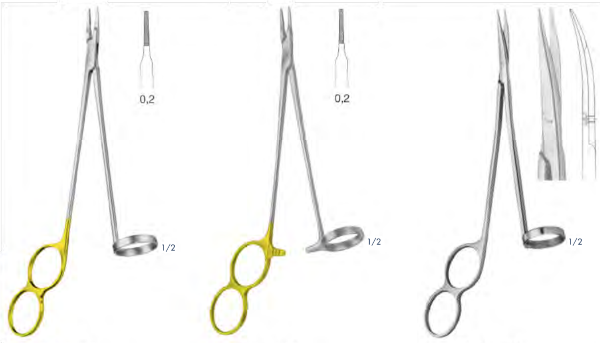
REIN/KUPKA ASI170370 Needle holder 190 mm
