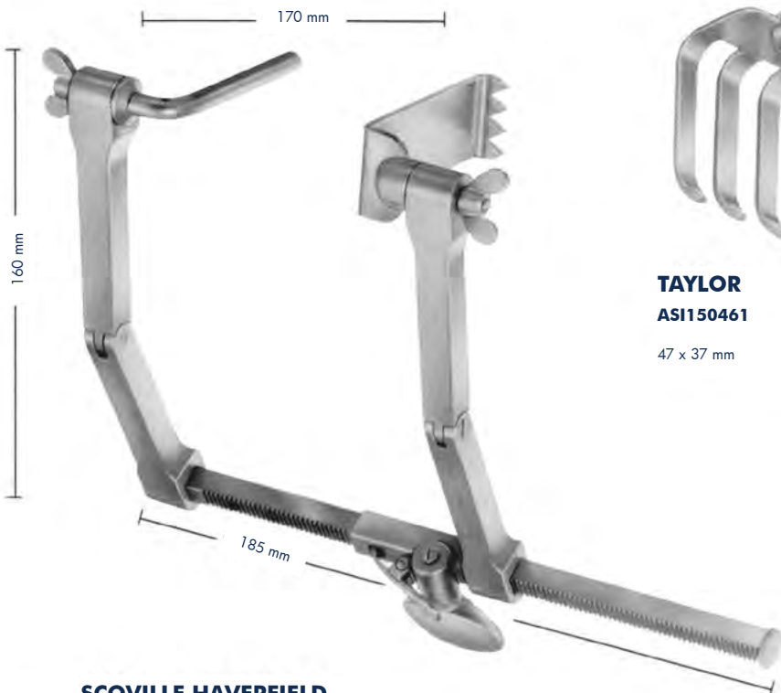
SCOVILLE HAVERFIELD ASI150453
