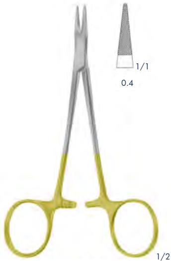
HALSEY ASI170328 130 mm
